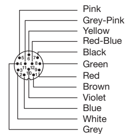
12 pin, M12 Cable Plug (Female)
