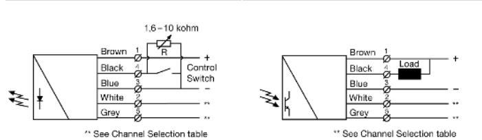
SMT 90X0C Variable range & test input setup
