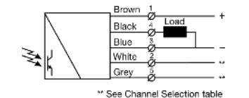
SMR 9XX0 Transistor PNP
