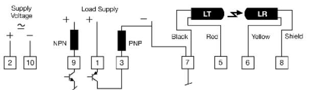
Transistor output – PA 11 A/B 40XT
