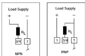
Transistor output – MPA 21 A/B 60X
